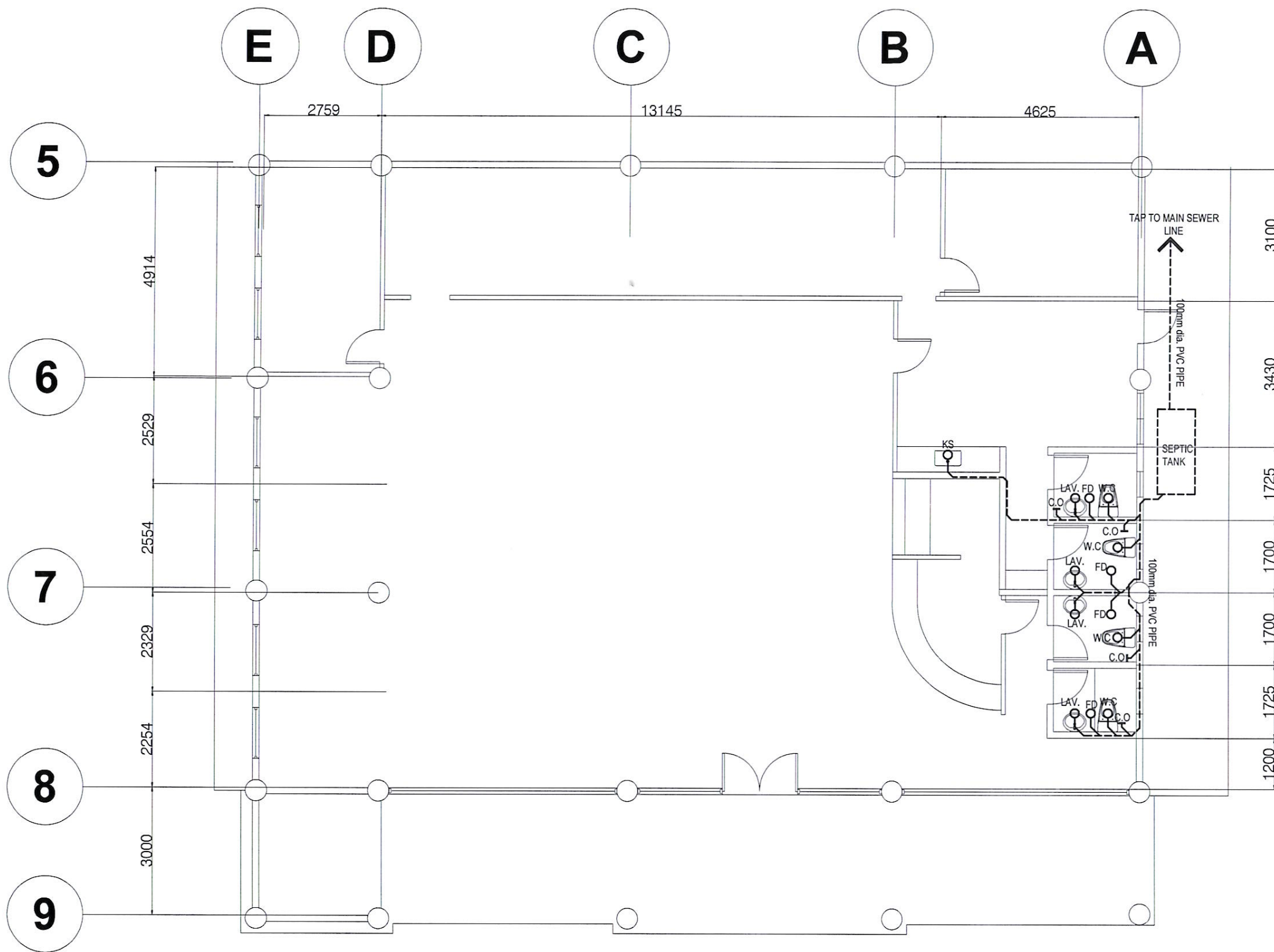
1 SEWER LINE LAYOUT P2/P2 SCALE 1:100mts
