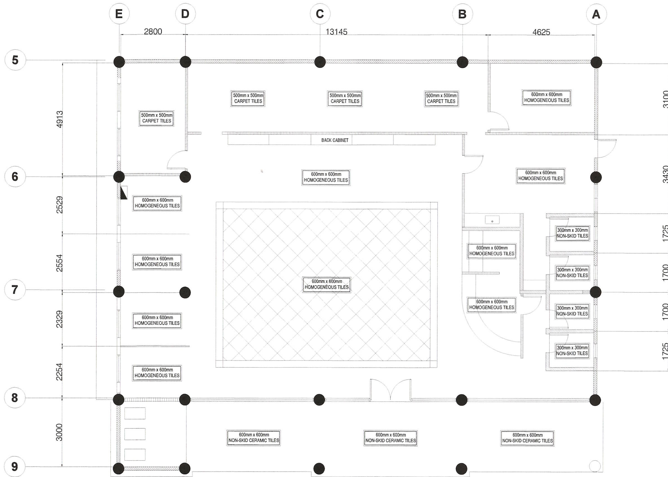
1 FLOOR PATTERN PLAN A6 A6 SCALE 1:90mts
