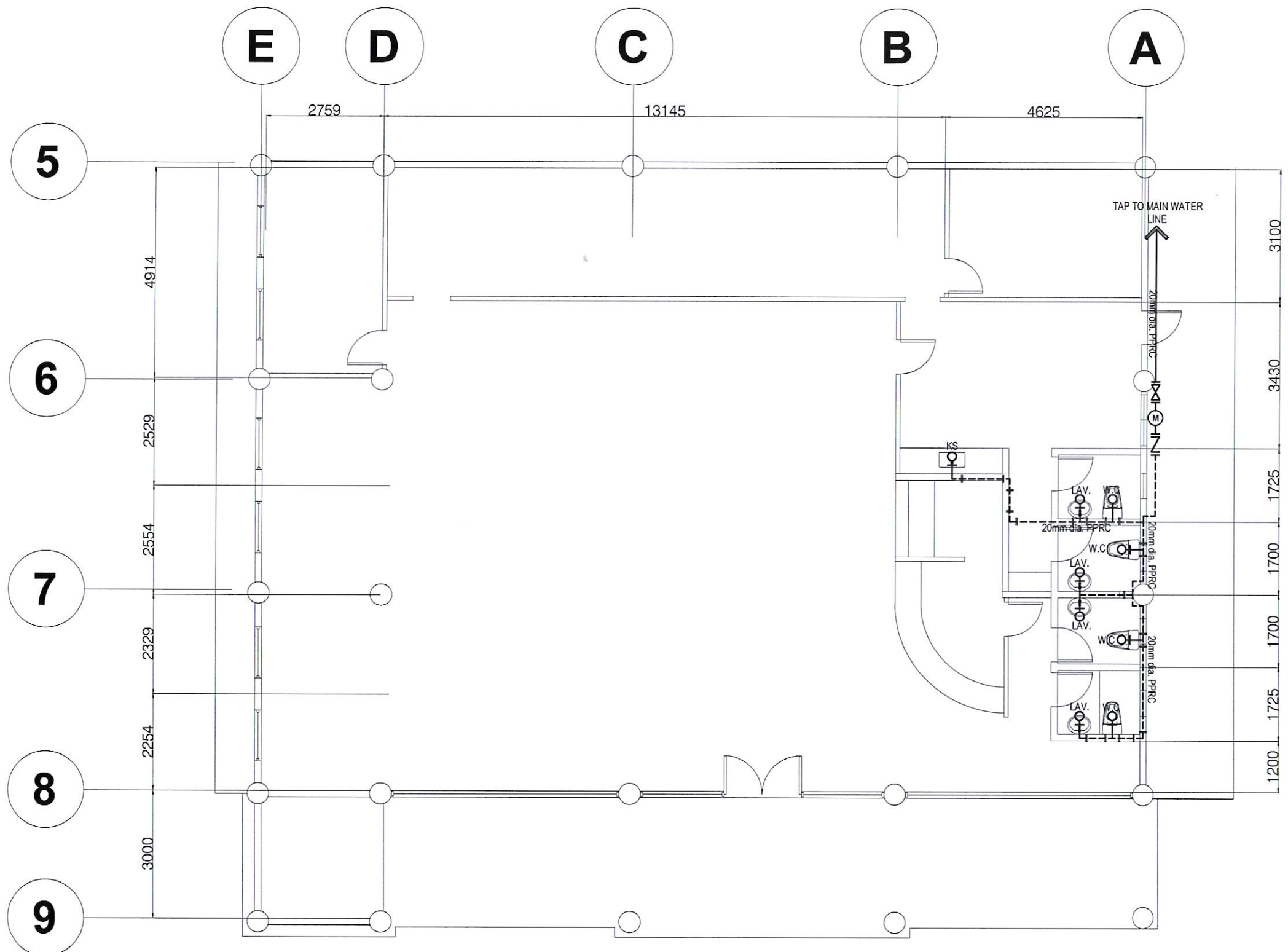
1 WATER LINE LAYOUT P1/P1 SCALE 1:100mts
