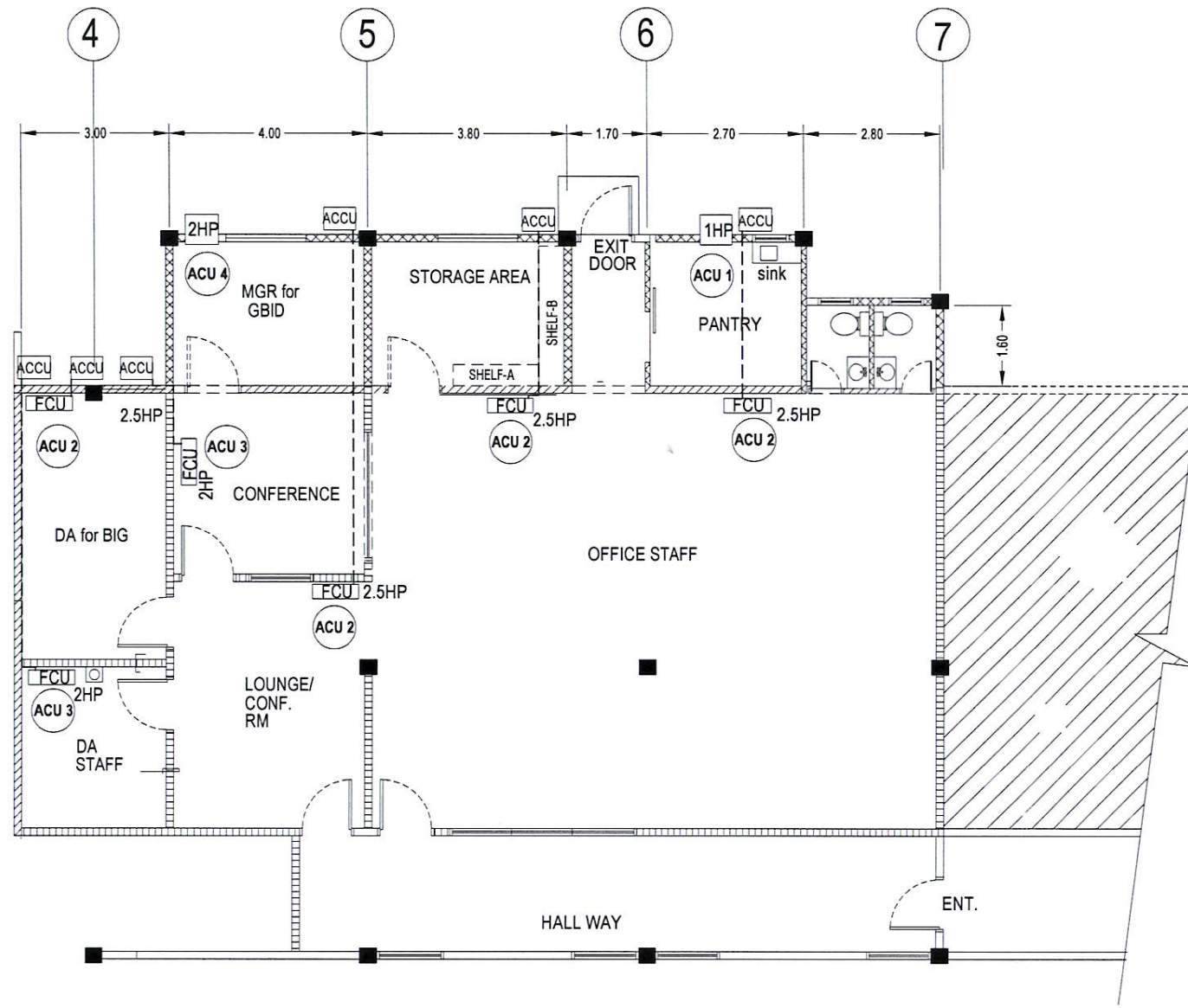
1 AIRCONDITIONING LAYOUT M-1M-1 SCALE: NTS
