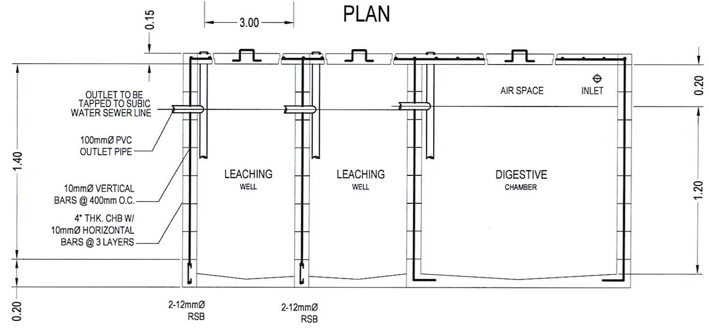
1 SEPTIC TANK DETAIL P1 P2 SCALE : 1:20 M
