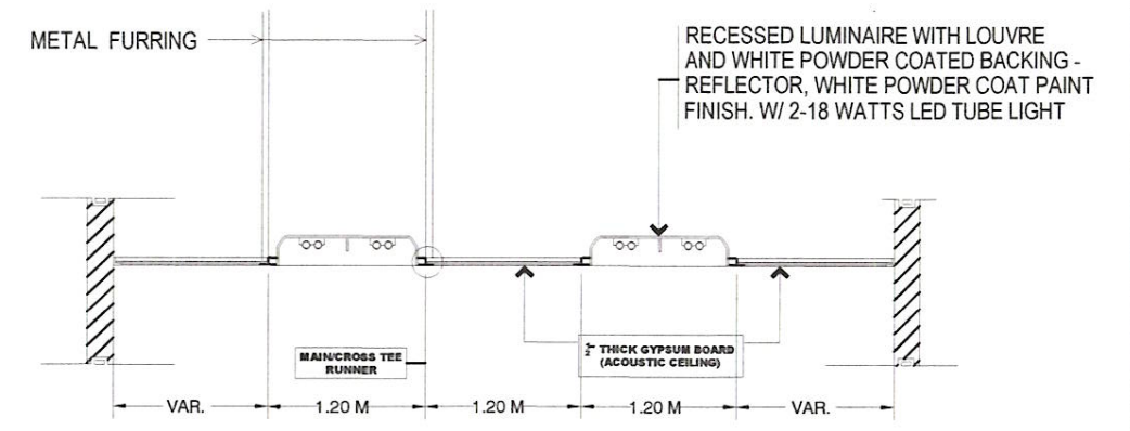
2 SECTION OF LIGHTING DETAIL A6 A6 SCALE 1:50 METERS
